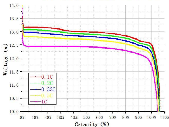
Different Rate Discharge Curve@25°C
