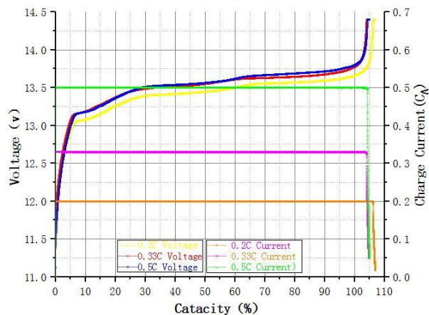
Charge Characteristics@25°C
