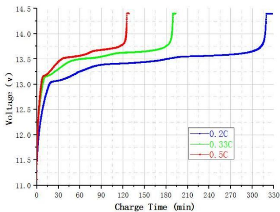
Charge Characteristics@25°C
