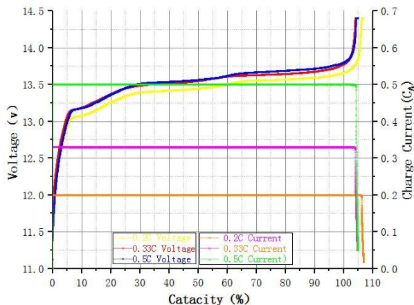
Charge Characteristics@25°C
