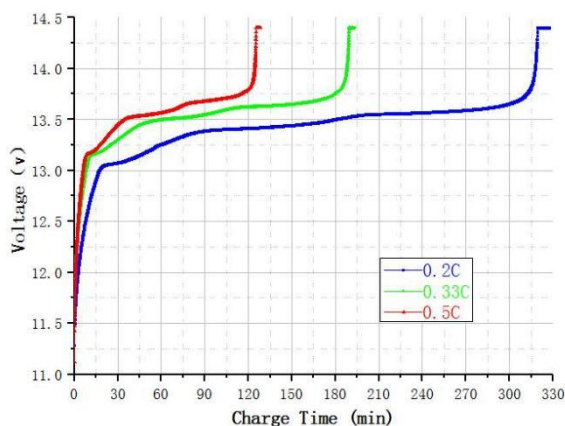
Charge Characteristics@25°C
